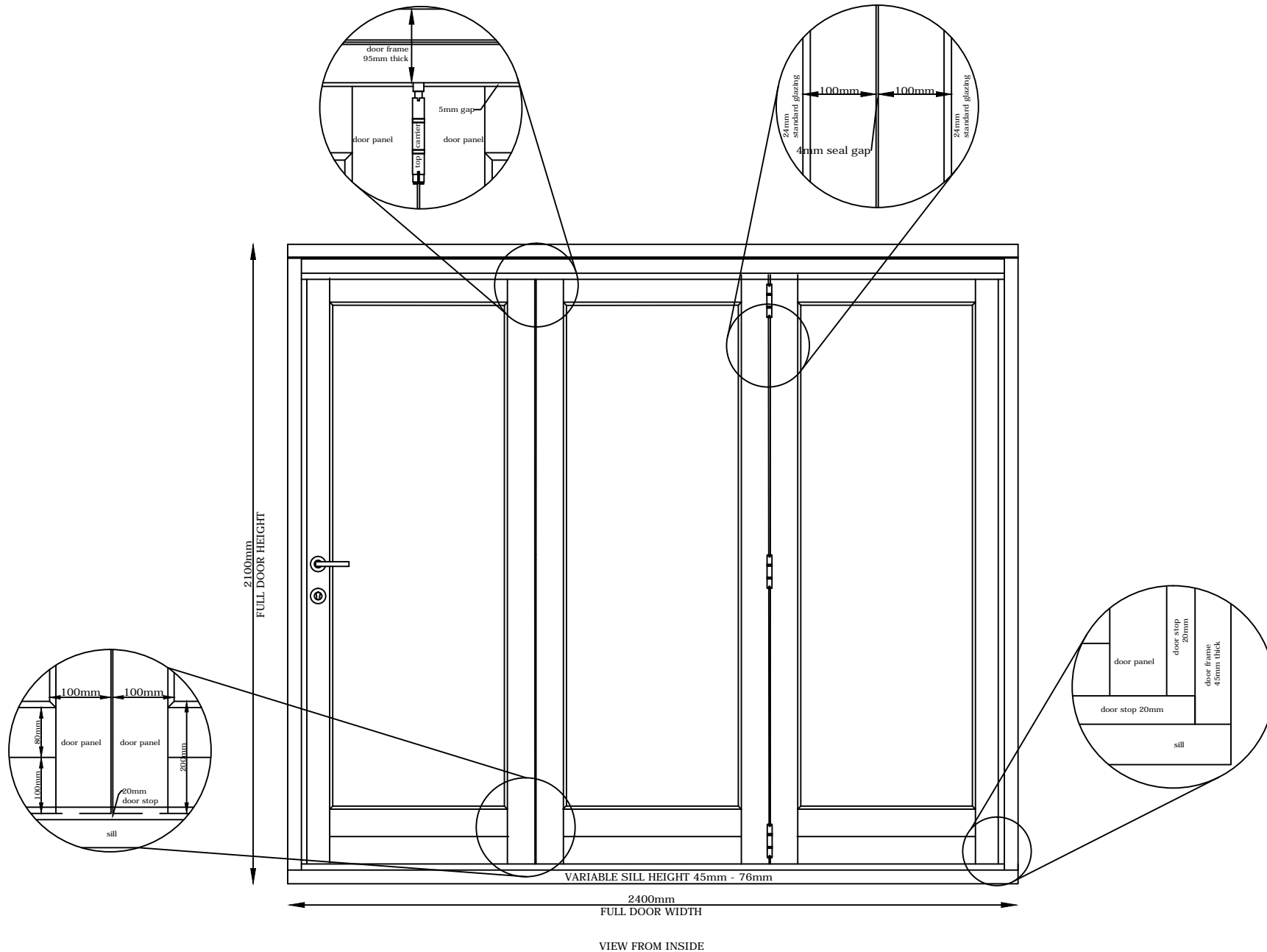
E3 Folding sliding door elevation - closed view from inside
